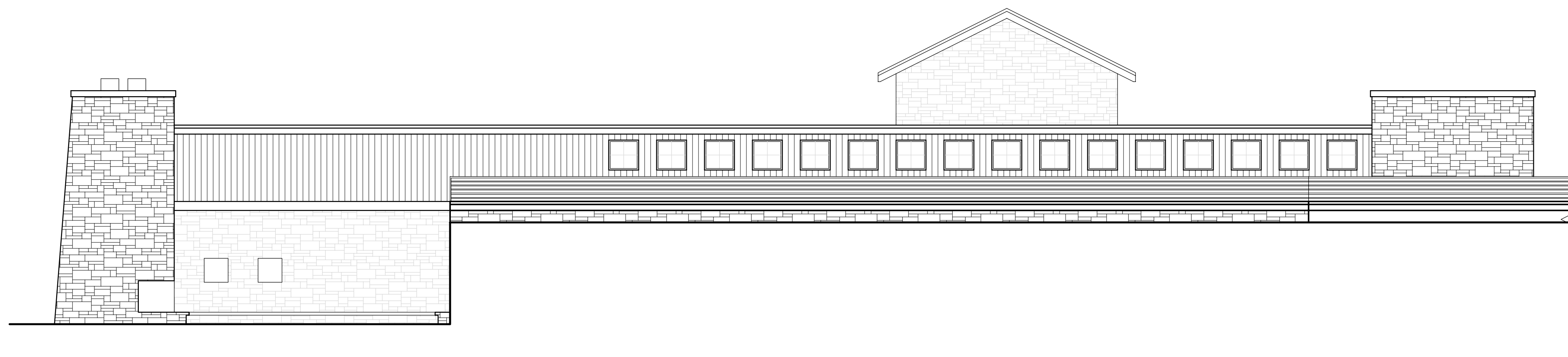
RIGHT WING - HILL ELEVATION
